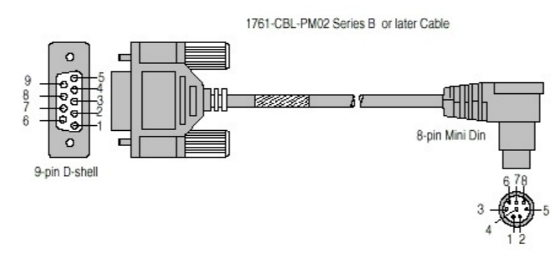
1761-CBL-PM02 Series B (or equivalent) Cable Wiring Diagram
